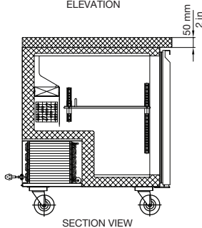
SECTION VIEW
