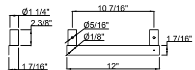
DETAIL "B"
