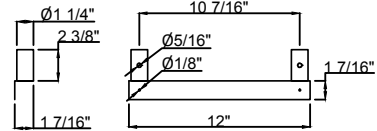
DETAIL "B"
