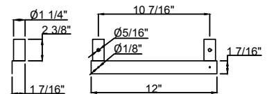
DETAIL "B"
