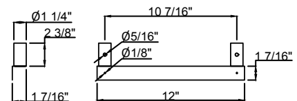
DETAIL "B"
