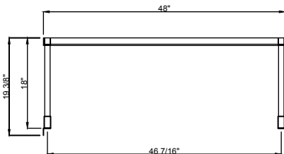
FRONT ELEVATION
