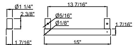
DETAIL "B"
